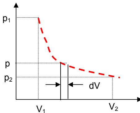
Irreversible process
